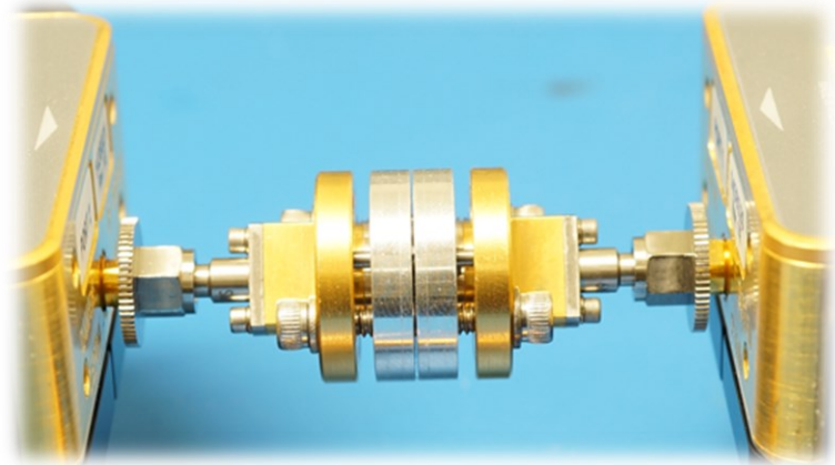
WAVEGUIDE TWIST, COMPACT
