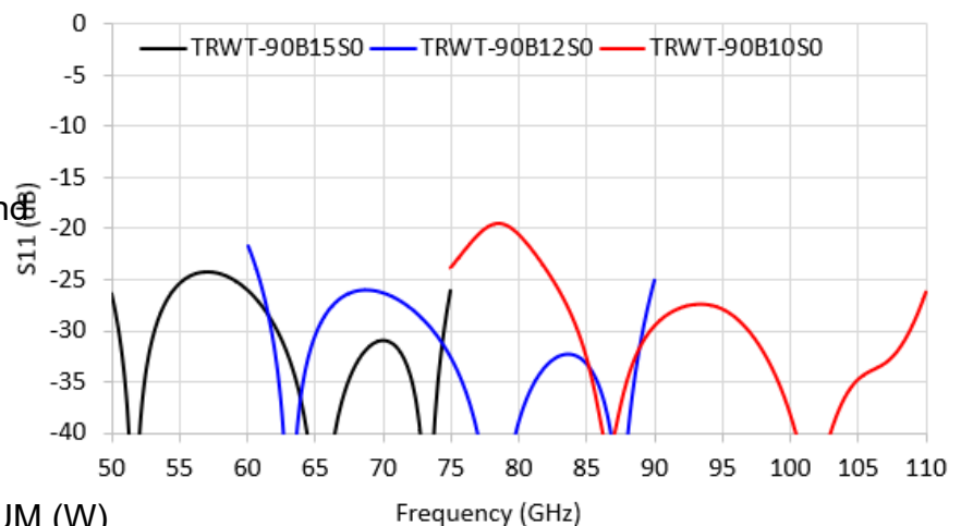
WAVEGUIDE TWIST, COMPACT
