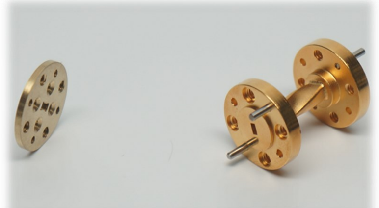
Comparison: Raytech's TRWT-90A Shim vs standard 1" Twist
