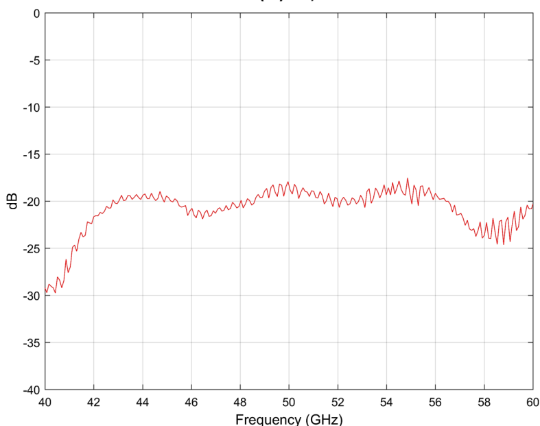
TRCW-198F(M)RC0, Reflection:
