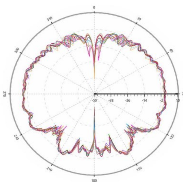
Elevation Cut: 40:0.25:43 GHz
