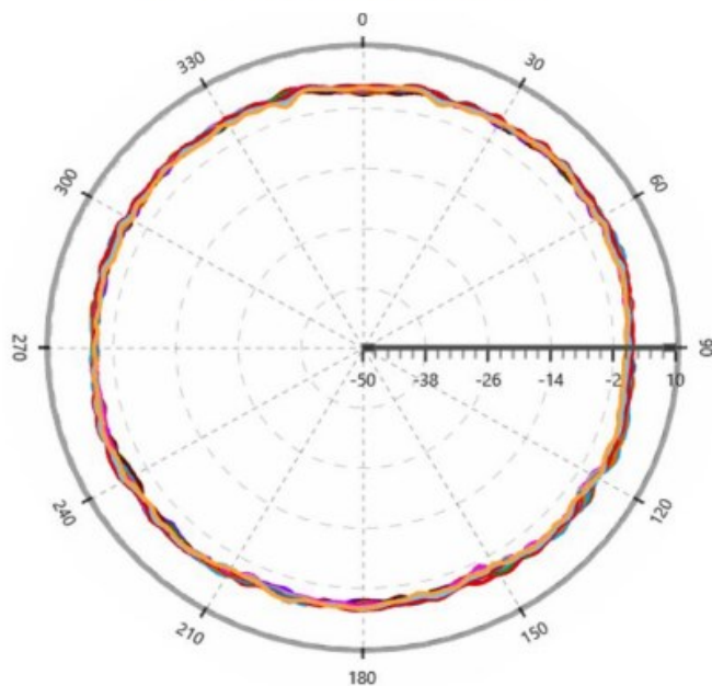
Azimuth Cut: 40:0.25:43 GHz
